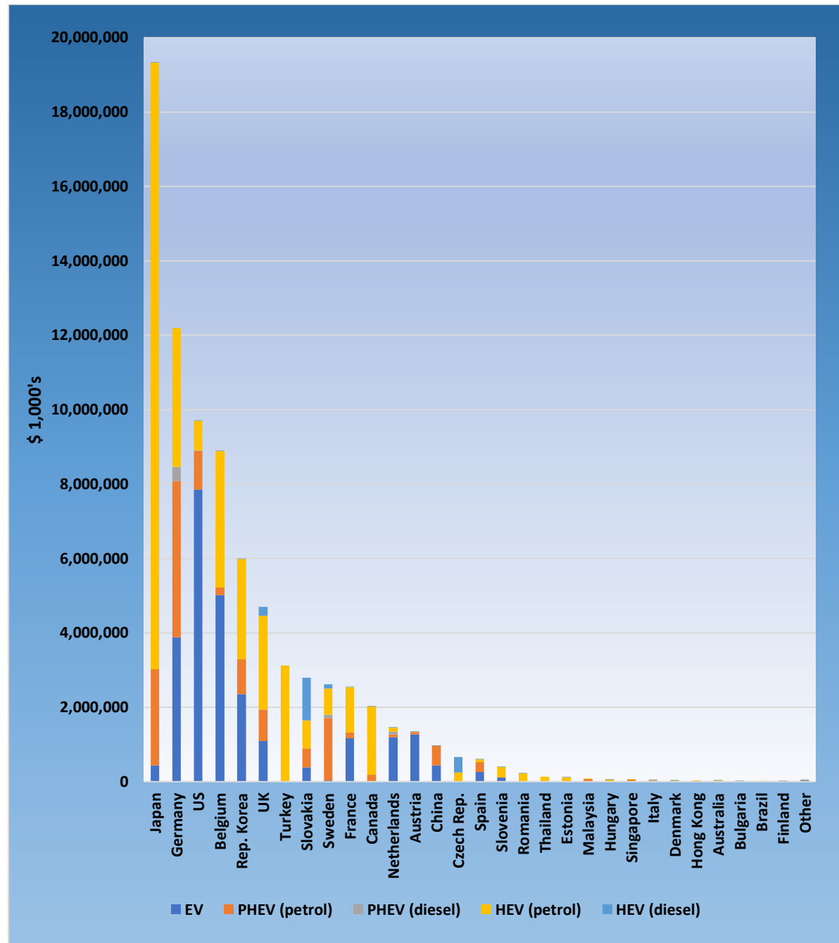
Figure 14.1 Top 30 Electric & Hybrid Vehicle (X)EV Exporting Countries 2019 ($ 1000's)
