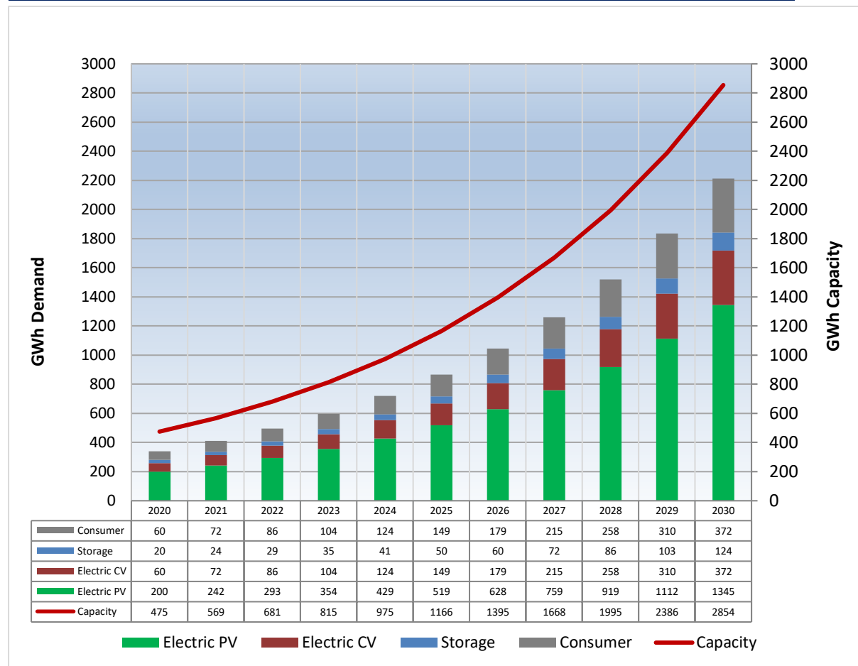
Figure 3.5 Global Lithium Battery Demand & Capacity Forecast by Sector 2020-2030
